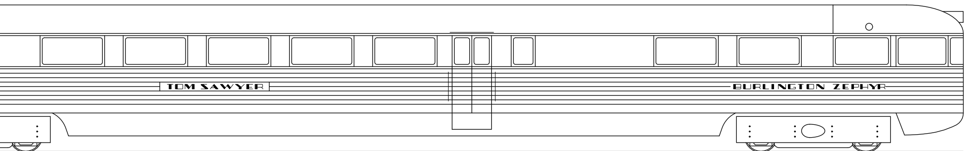
#572 L.O.A. 75'5" WHLB. 64'0"
