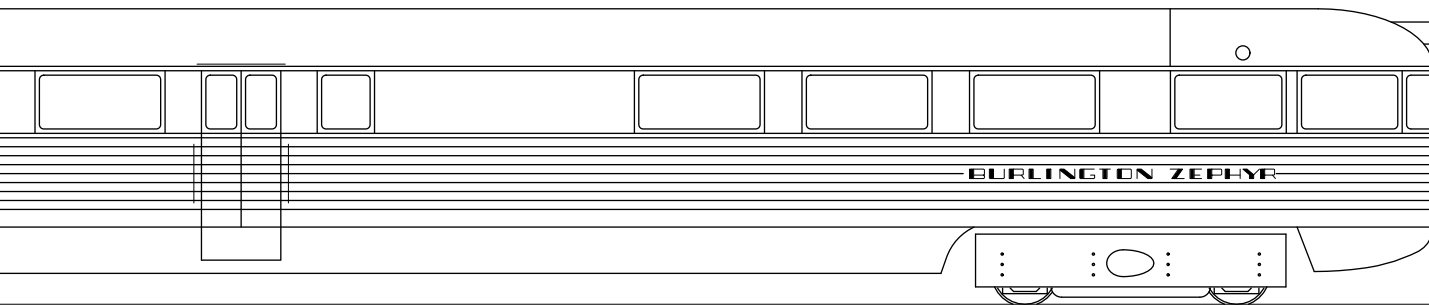
02 L.O.A. 70'0" WHLB. 58'7"
