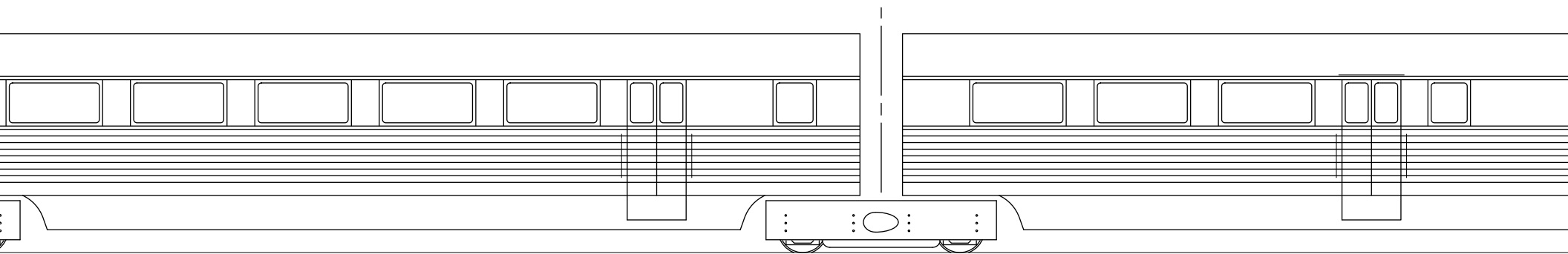
#525 L.O.A. 49'8-1/2" WHLB. 49'8-1/2"
