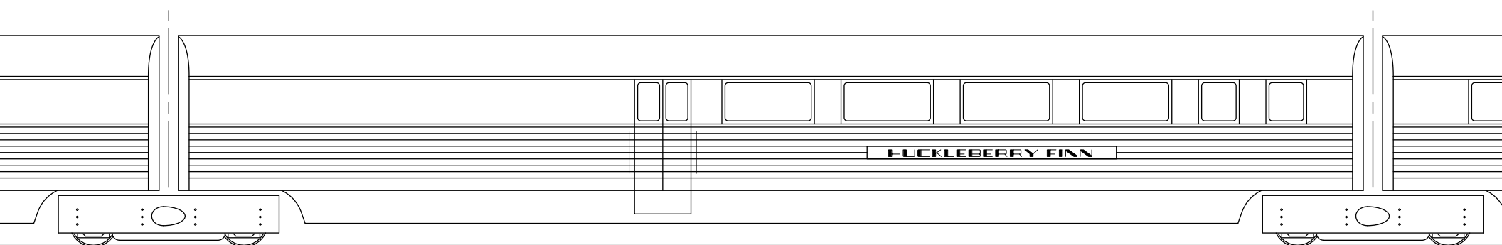
#551 L.O.A. 64'0" WHLB. 64'0"
