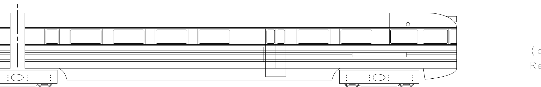
L.O.A. 64'9-1/2" WHLB. 53'4-1/2"
