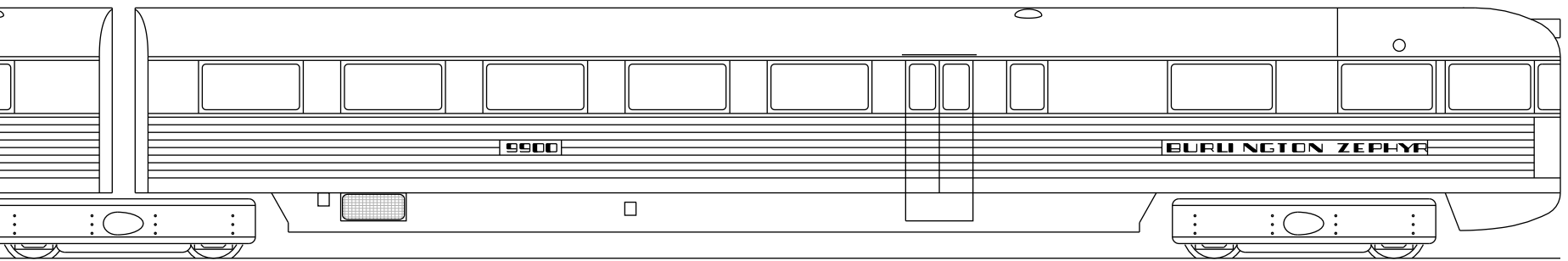
Car 570 - L.O.A. 63'10" WHLB. 52'7"
