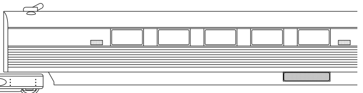
Car 500 - L.O.A. 64'0" WHLB. 64'0"
