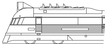
(Cabroof vents added ~1938 Main lights added ~1949)
