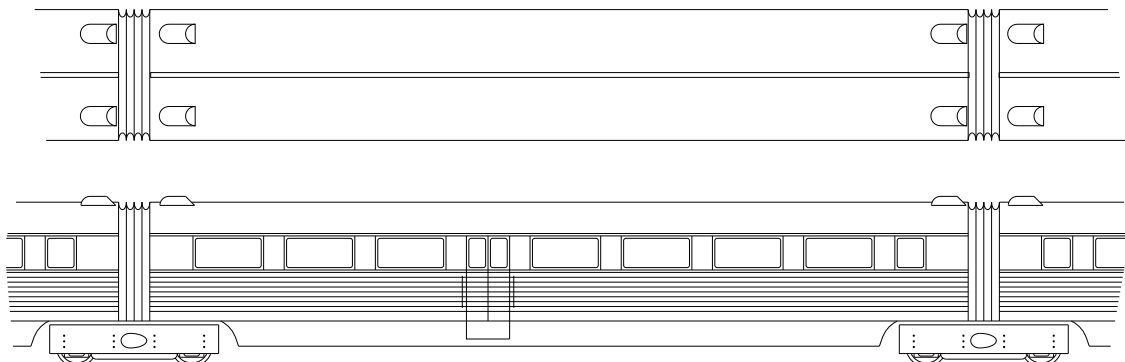
L.O.A. 59'0" WHLB. 59'0"
