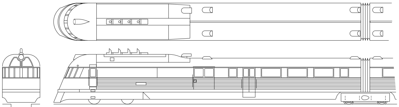
L.O.A. 75'3" WHLB. 61'5-1/4"
