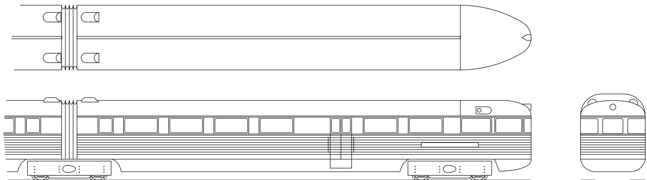
L.O.A. 64'9-1/2" WHLB. 53'4-1/2"
